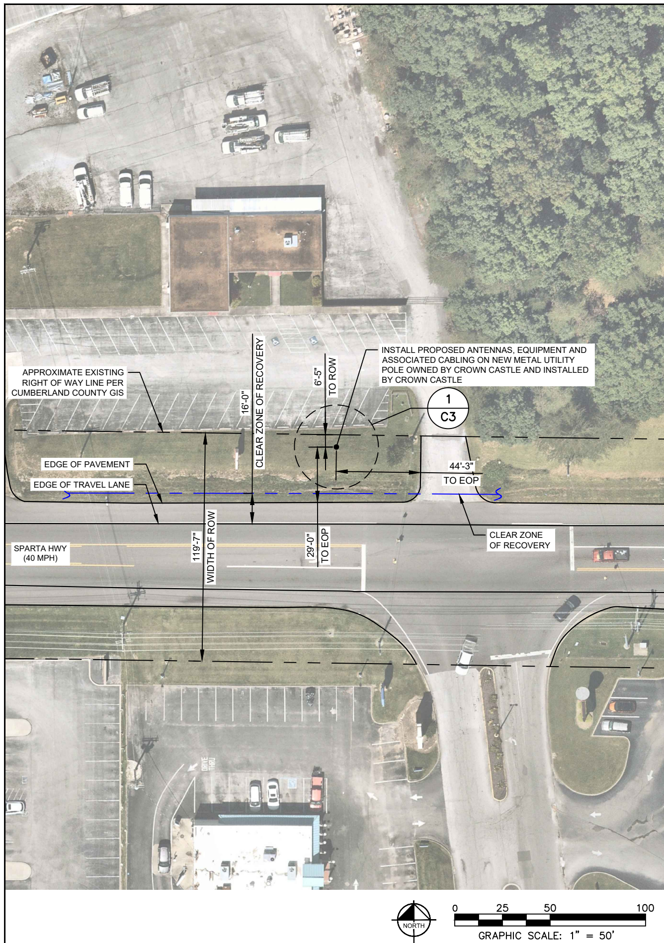
PROPOSED NODE LOCATION PLAN
