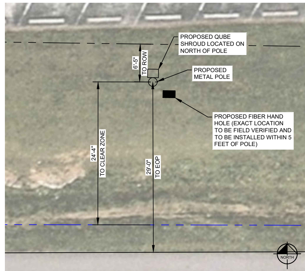
1 EQUIPMENT DETAIL C3 SCALE : 1" = 10'
