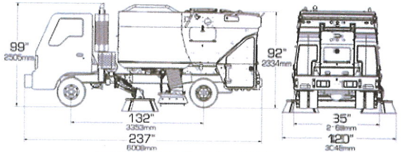
*TYPICAL MEASUREMENTS SHOWN. EXACT DIMENSIONS DEPENDING ON OPTIONS AND TRUCK MANUFACTURER
