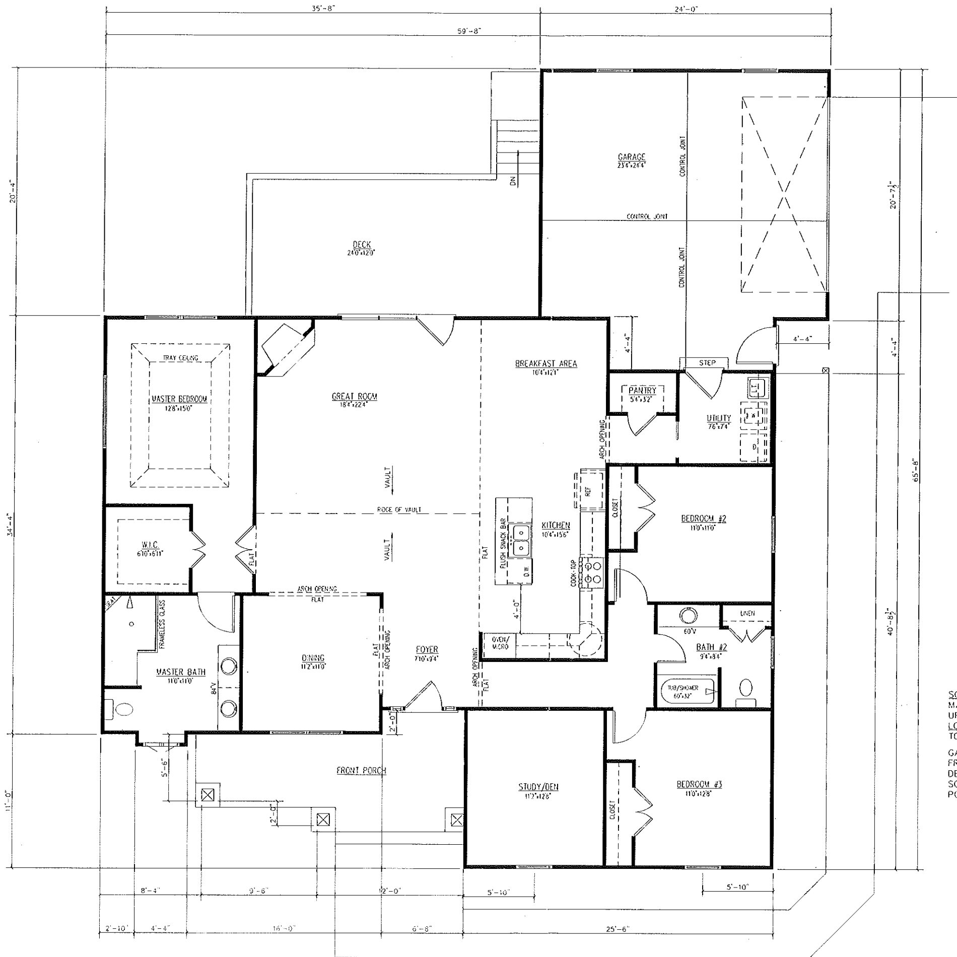
FLOOR PLAN 1/4"=1'-0"
