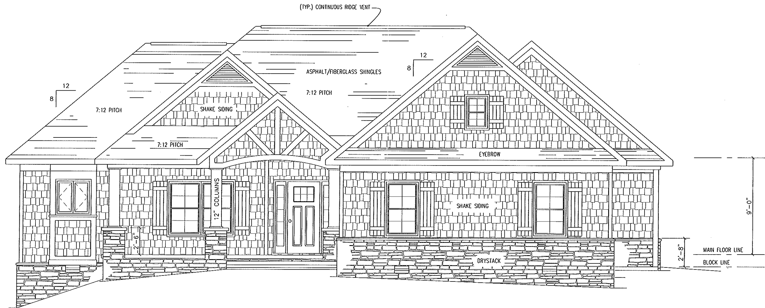
FRONT ELEVATION 1/4"=1'-0"
