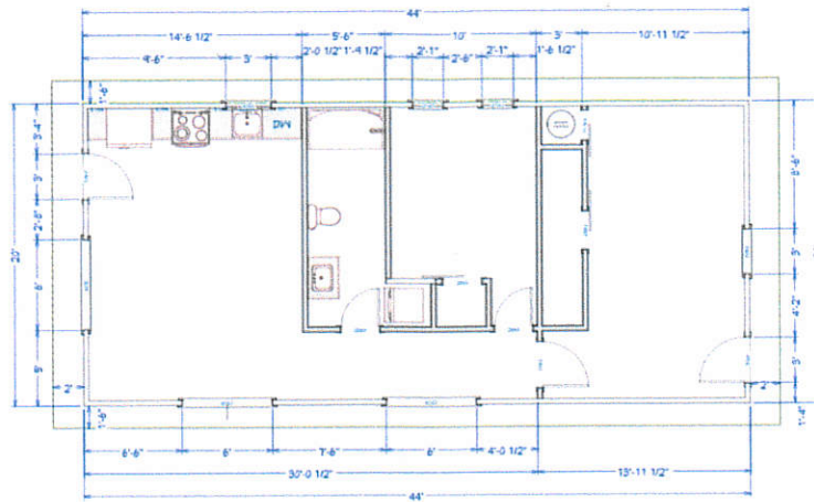
LIVING AREA 550 SQ. FT.
